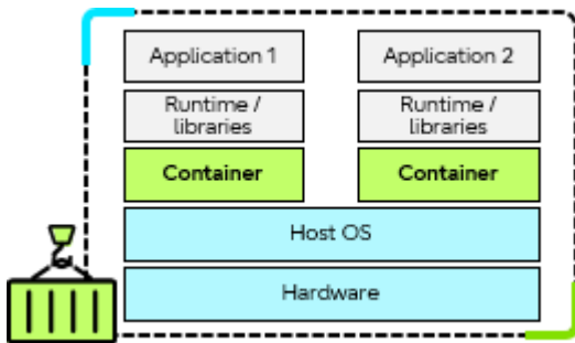
Containers save resources by sharing the kernel of the host OS
